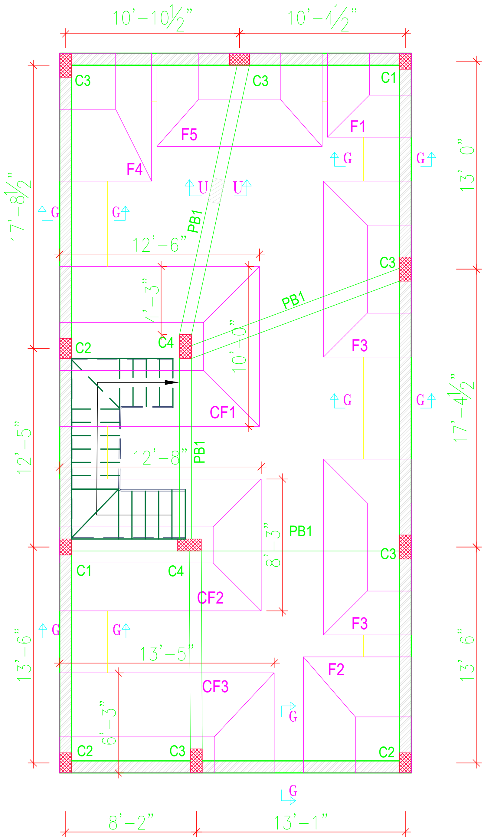
FOUNDATION PLAN
